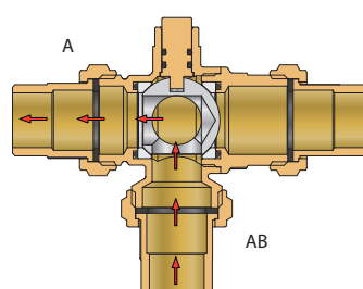
CLOSED ACTUATOR
