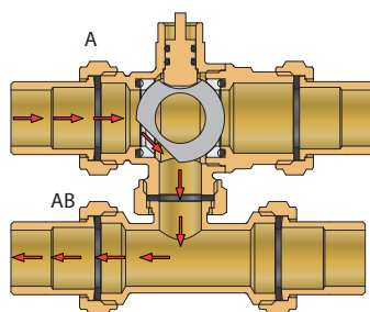
CLOSED ACTUATOR
