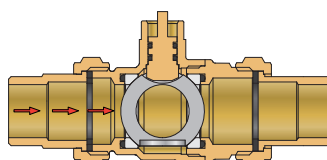
CLOSED ACTUATOR
